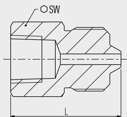
Female-male connection adapter Nominal pressure: 15,000 psi [1,034 bar]
