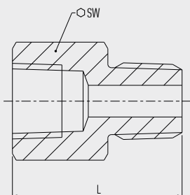
Female-male connection adapter Nominal pressure: 15,000 psi [1,034 bar]
