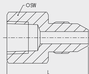
Female-male connection adapter Nominal pressure: 15,000 psi [1,034 bar]
