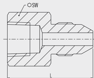
Female-male connection adapter Nominal pressure: 15,000 psi [1,034 bar]
